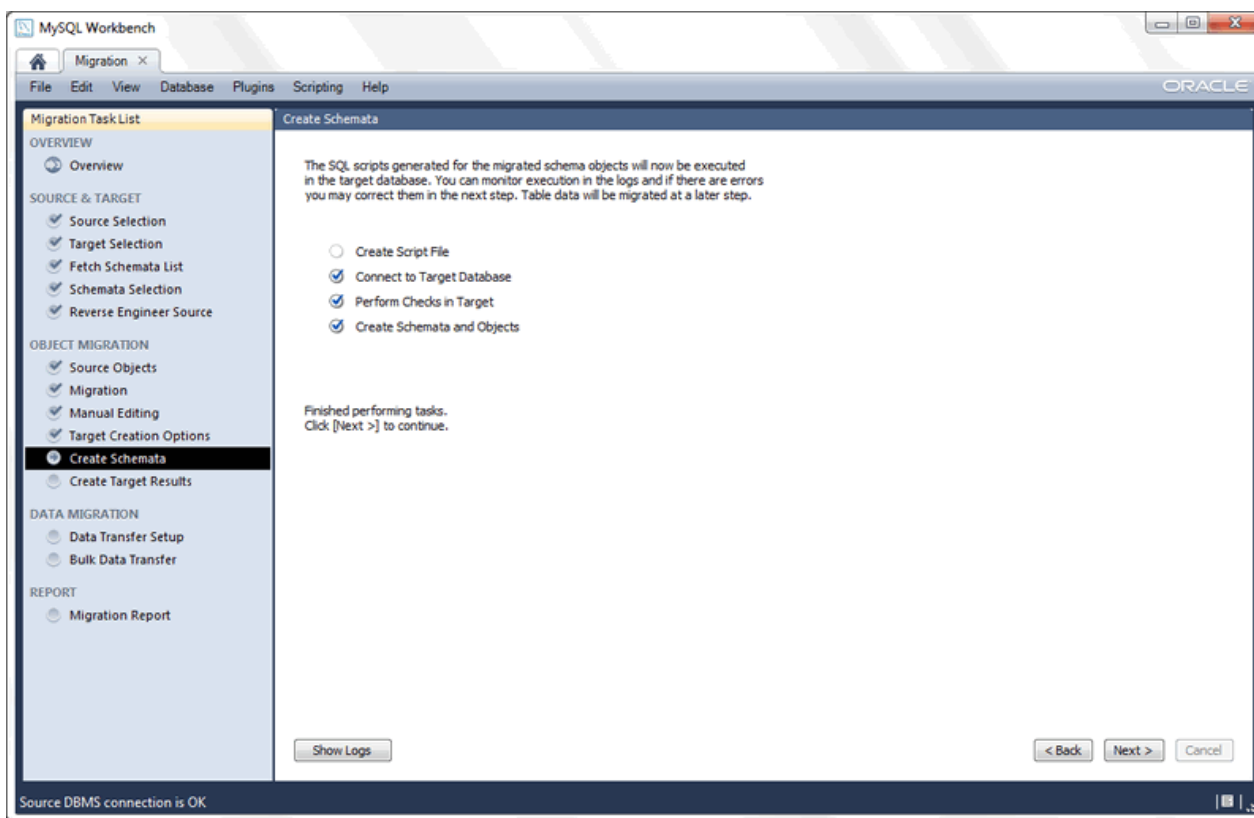
Figure 10.34 Create Schemas
